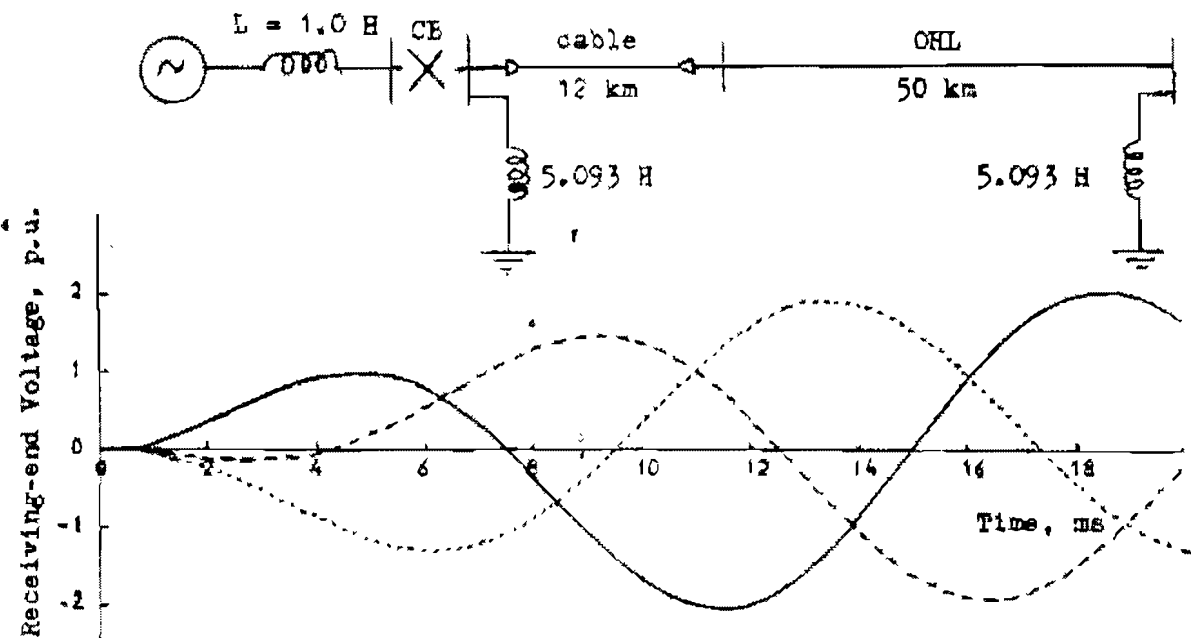
Fig. 5: Effect of shunt-reactor compensation at both sending and receiving ends on the receiving-end voltage. Maximum value = 2.044 p.u.
