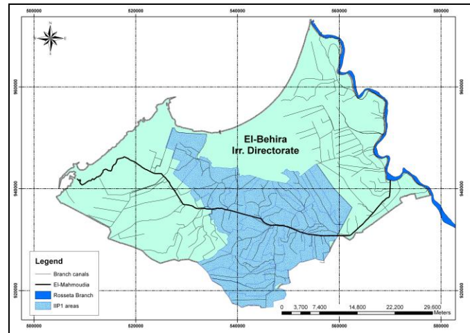
Figure 2: El-Mahmoudia command area and its improved area
