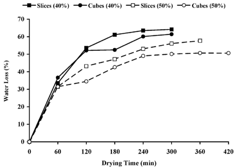
Fig. (5): Water loss (WL%) for osmotic-air dried apples (slices and cubes) in 40 and 50% sucrose solution
