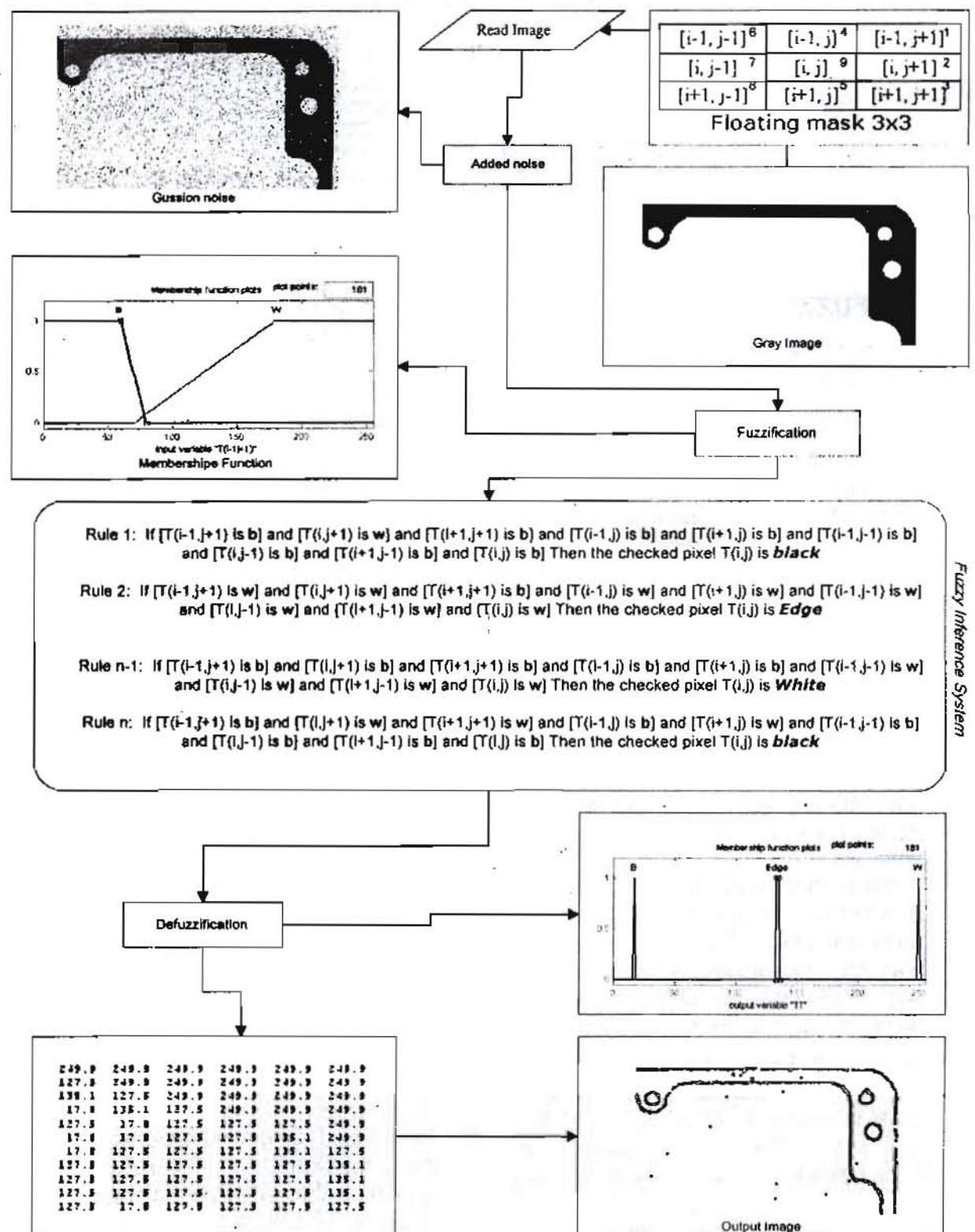
Fig.2. The Proposed Fuzzy Filter and Edge Detection Flow chart
