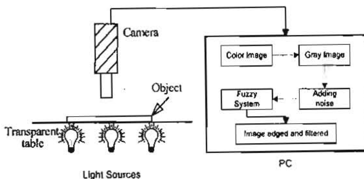
Fig.1 Vision System
