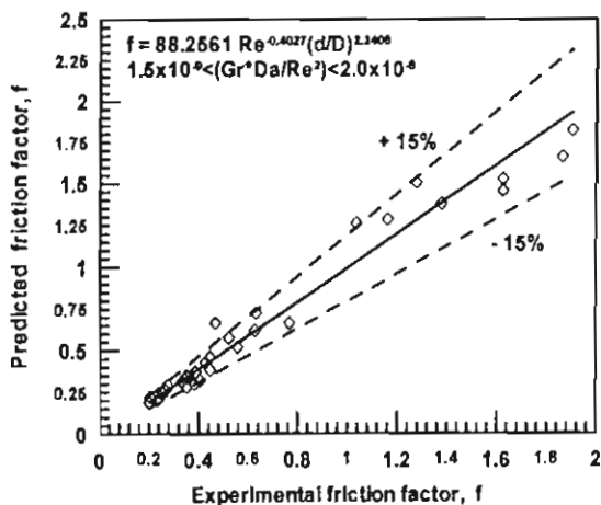
Fig. (10) Correlation of present experimental data of friction factor with the predicted results.
