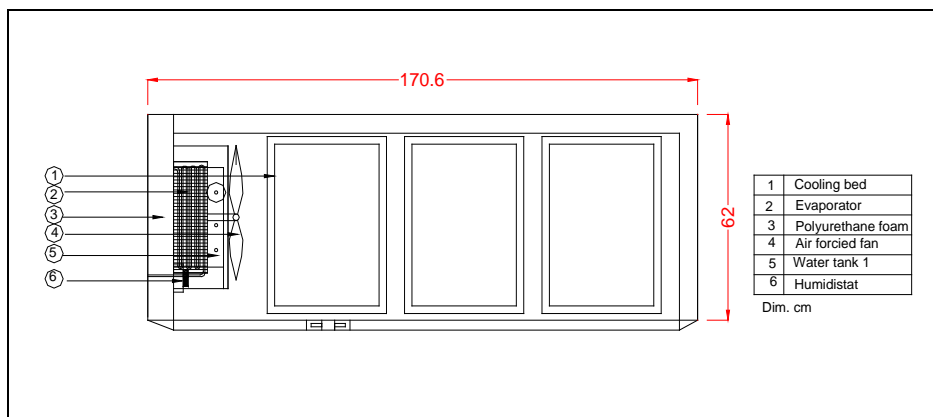
Fig. (2): Schematic diagram of the cooling chamber.
