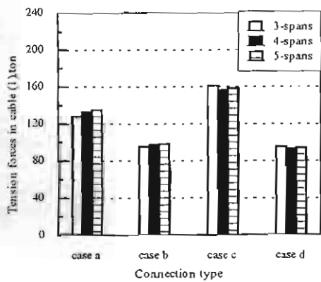
Fig.(8-a):Tension forces in cable (1) in suspension bridge
