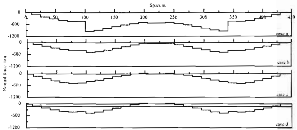
Fig (17-c). Normal force along floor beam in cable stayed (radiating) bridge.
