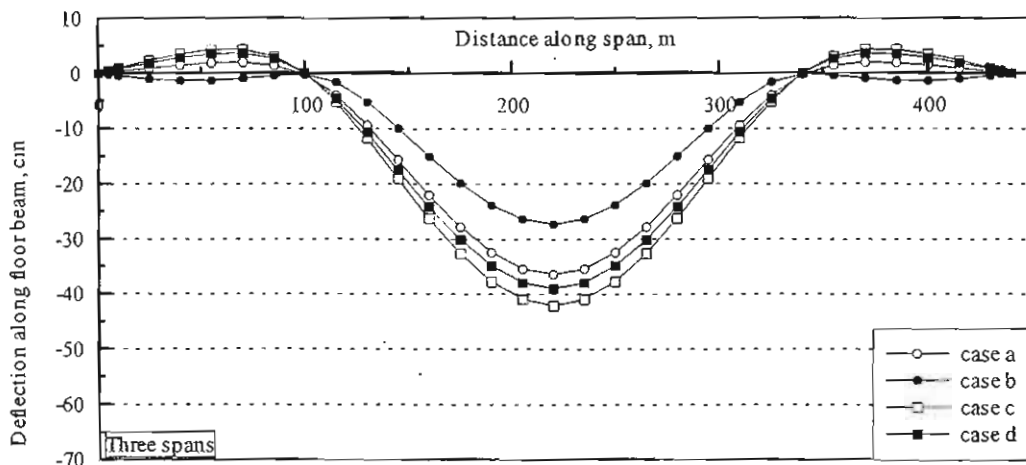
Fig.(10-c): Variations of deflections along floor beam in cable stayed (rading) bridge.
