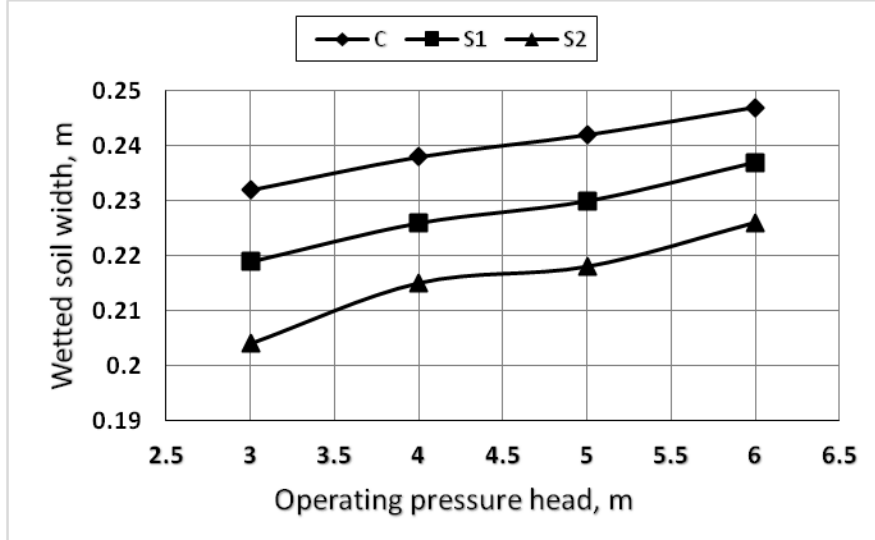
Figure2:Effect of operating pressure head on horizontal wetting zone (wettered soil width).
