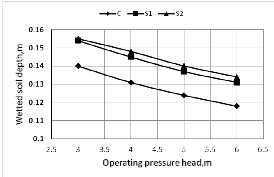
Figure 3:Effect of operating pressure head on vertical wetting zone (wettered soil depth).
