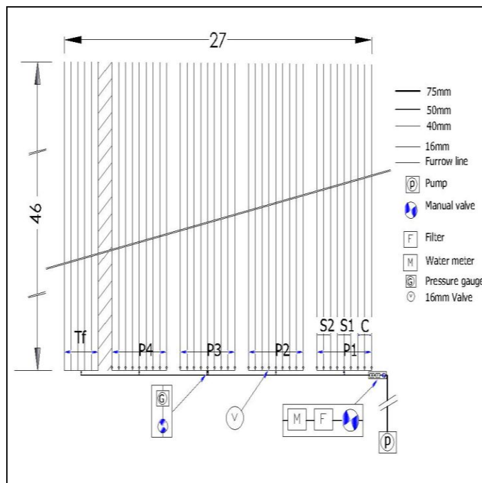
Figure 1: Layout of irrigation systems with the experimental design
