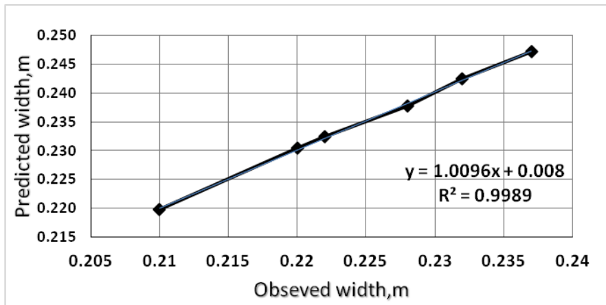
Figure4: The relationship between observed and predicted wetting width.
