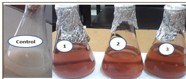
Picture 1. Chang in color to brown indicated to the synthesis of AgNPs. Supernatants (1, 2 and 3) treated with silver nitrate. Control as a supernatant silver nitrate free. 1. Supernatant of Potato dextrose broth medium, 2. Supernatant of Sabouraud broth medium and 3 Supernatants of malt yeast broth medium.
