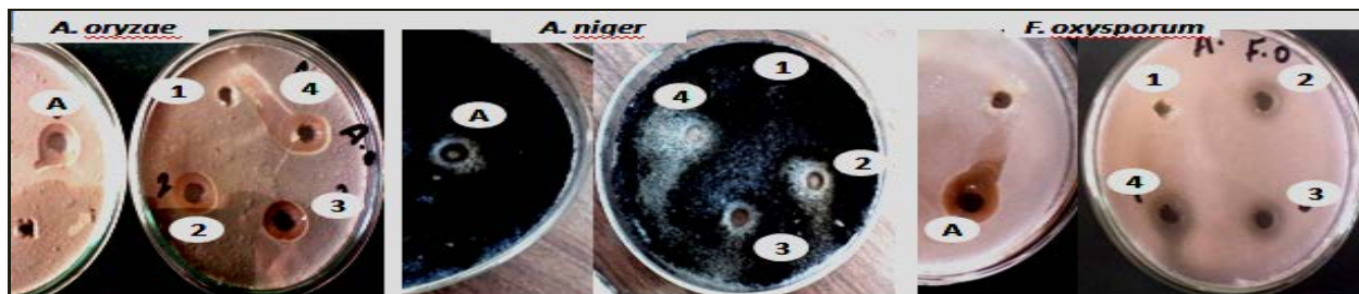
Fig. 5. Antifungal activity of the synthesized AgNPs. (1) represents \text{AgNO}_3 , Numbers 2, 3 and 4 represent AgNPs synthesized using supernatant of media 1, 2 and 3, respectively- (A). Antifungal drug nystatin.
