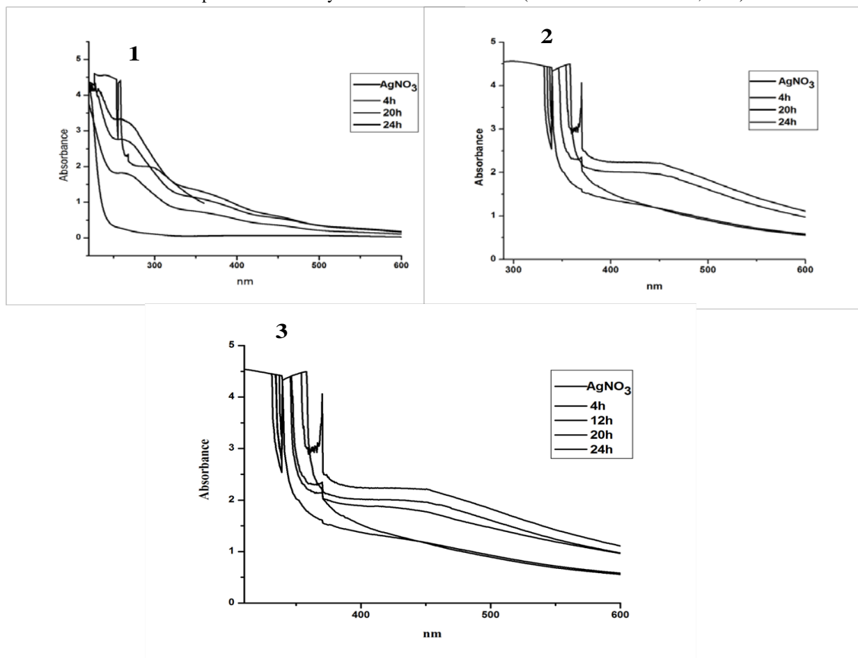
Fig. 1. UV-visible spectra of the synthesized AgNPs by supernatants of growing F. oxysporum on different culture media: 1. potato dextrose broth medium, 2. Sabouroud broth medium and 3. Malt yeast broth medium.
