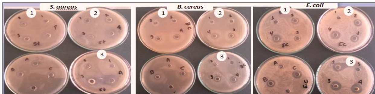
Fig.4. Antibacterial activity of different volumes of AgNPs synthesized using supernatants of growing F. oxysporum on different culture media The numbers of wells 1, 2, 3 and 4 represents the volume of AgNPs 10, 20, 50 and 100 µl – A: a pure AgNO 3 , B: Erythromycin and C: Ofloxacin for each S. aureus and B. cereus and B: Norfloxacin, C: Ofloxacin for E. coli .
